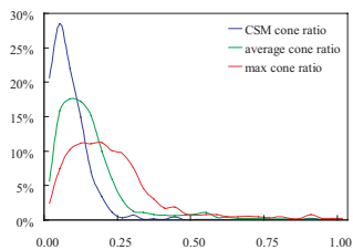
Fig. 2 Histogram of cone ratio.
