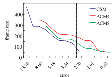
Fig. 3 Comparisons of error and frame rate among CSM, ACM4 (4-sector ACM) and ACM8 (8-sector ACM).
