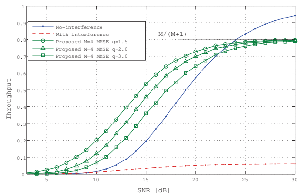
Fig. 6. Throughput performance with MMSE criterion ( M = 4, q = 1.5, 2, 3 )
