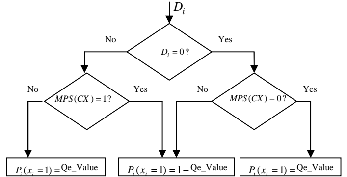
Fig. 3 Flow chart of the proposed method to estimate the local PMF: P_i(x_i = 1) on the i^{\text{th}} bit-plane; CX denotes the context of the input; D_i
